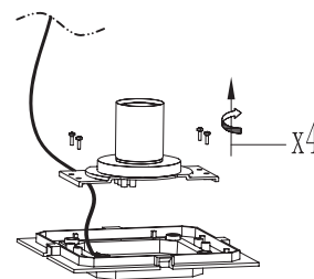
Untie screws
