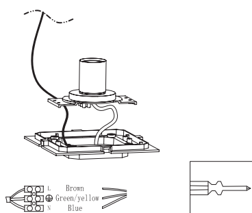
Connect wires
