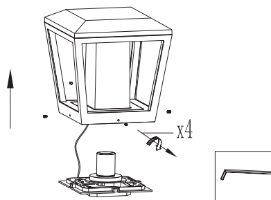
Dismantle parts by untying screws
