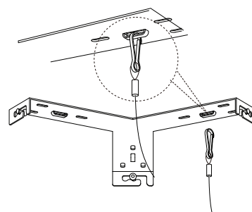
Make it stable
