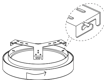
Adjust the wire & fix it into place
