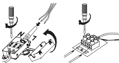
Connect the wires
