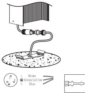
Connect wires
