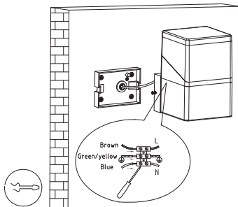
7. Connect the wires.
